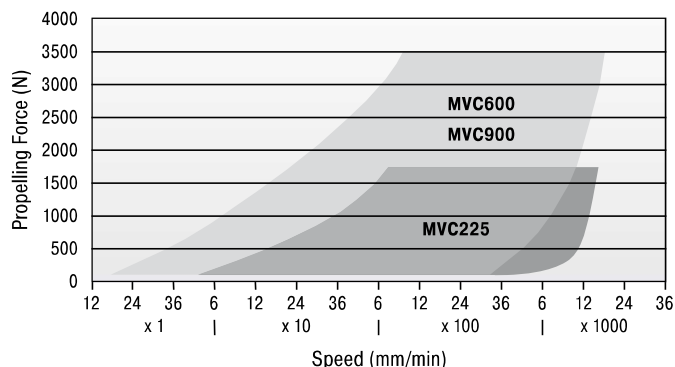
Operating Range MVC225 to MVC900
